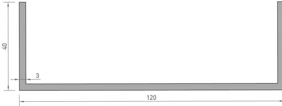
8601 U PROFİLİ 1,577 kg/mt
