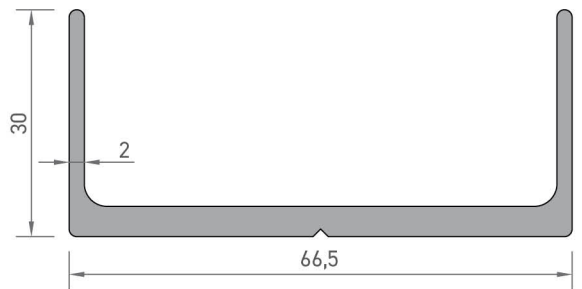
4632 U PROFİLİ 1,007 kg/mt
