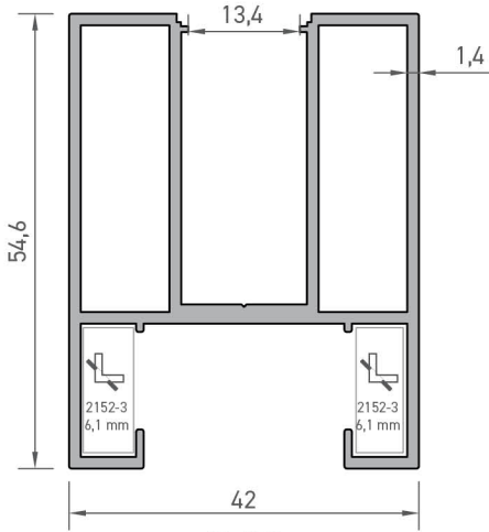
8780 KASA PROFİLİ 1,030 kg/mt
