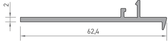
4151 DAYAMA PROFİLİ 0,395 kg/mt
