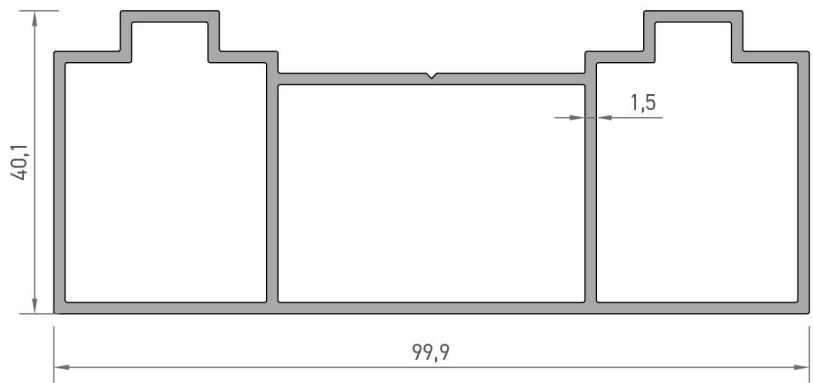
4153 DESTEK PROFİLİ 1,415 kg/mt
