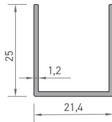
4515 MOBİLYA "U" PROFİLİ 0,230 kg/mt
