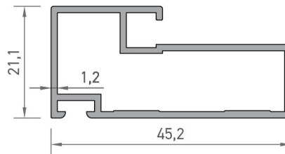
2970 MOBİLYA PROFİLİ 0,472 kg/mt
