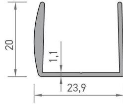
2100 MOBİLYA "U" PROFİLİ 0,230 kg/mt
