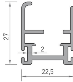
3070 MOBİLYA PROFİLİ 0,408 kg/mt
