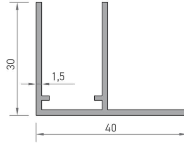
8198 MOBİLYA "F" PROFİLİ 0,407 kg/mt
