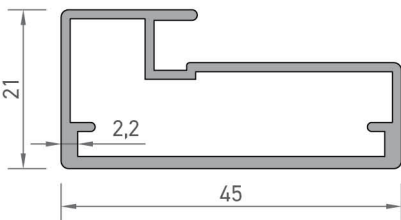
2846 MOBİLYA PROFİLİ 0,524 kg/mt
