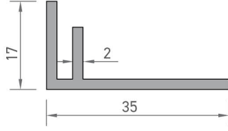
4120 MOBİLYA "F" PROFİLİ 0,325 kg/mt
