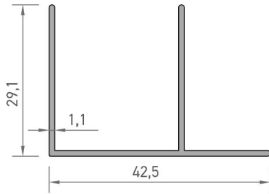
4981 MOBİLYA "F" PROFİLİ 0,295 kg/mt
