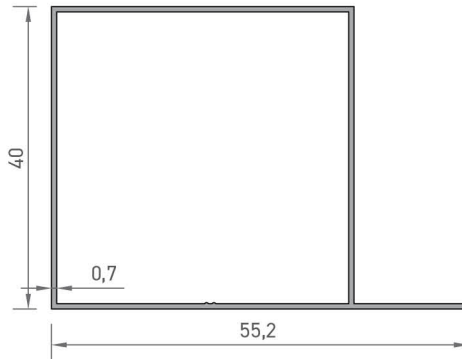
8414 MOBİLYA PROFİLİ 0,330 kg/mt
