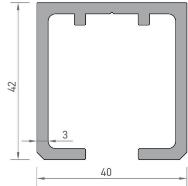
3208 ASKI RAY PROFİLİ 1,168 kg/mt
