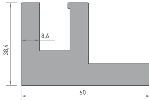
3397 MOBİLYA "F" PROFİLİ 3,195 kg/mt
