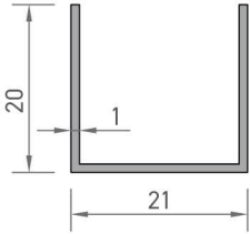
2859 MOBİLYA "U" PROFİLİ 0,160 kg/mt
