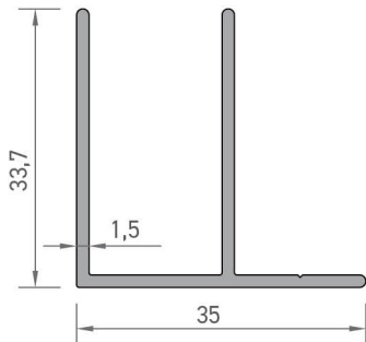
8883 MOBİLYA "F" PROFİLİ 0,401 kg/mt
