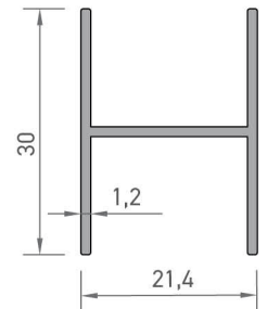
4517 MOBİLYA "H" PROFİLİ 0,260 kg/mt
