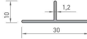
4516 MOBİLYA "T" PROFİLİ 0,125 kg/mt
