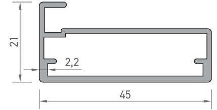
2845 MOBİLYA PROFİLİ 0,502 kg/mt
