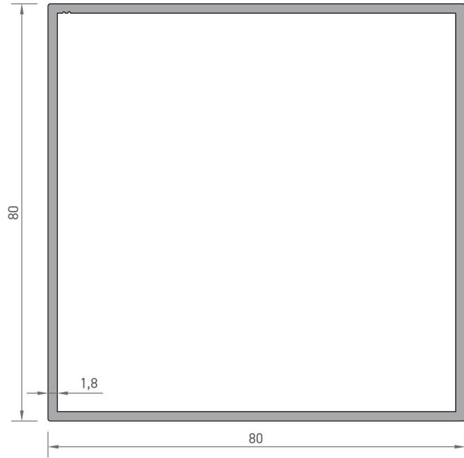
6644 KUTU PROFİLİ 1,525 kg/mt
