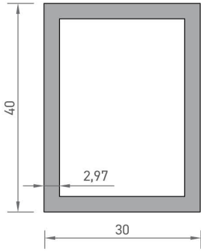
7817 KUTU PROFİLİ 1,041 kg/mt
