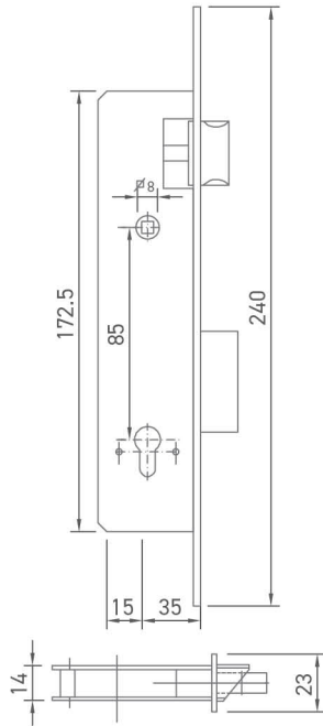
Geniş Kilit (Dilli) Wide Type Lock (Bolt) W55.780-1
