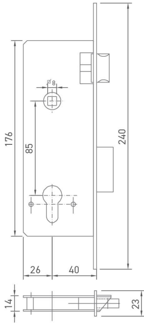
Geniş Kilit (Dilli) Wide Type Lock (Bolt) W55.780
