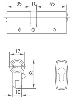
Barel Cylinders AT55.784
