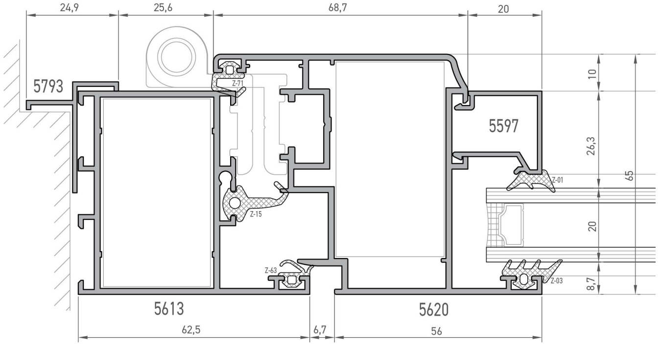
PVC Kanallı Kesit 9 mm PVC Groove Section 9 mm
