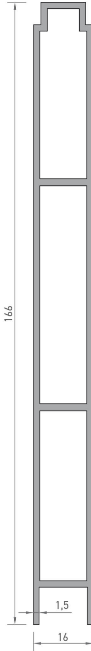
8870 TAHTA LAMBİRİ PROFİLİ 1,765 kg/mt
