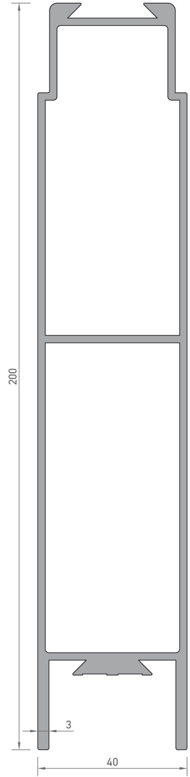
2964 TAHTA LAMBİRİ PROFİLİ 3,168 kg/mt
