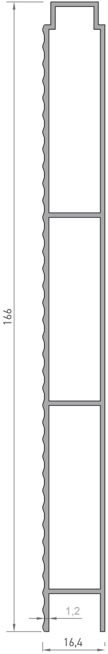
9288 LAMBİRİ PROFİLİ 1,329 kg/mt
