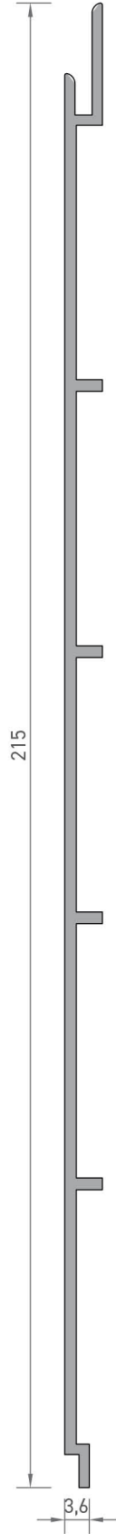
2117 LAMBİRİ PROFİLİ 1,095 kg/mt
