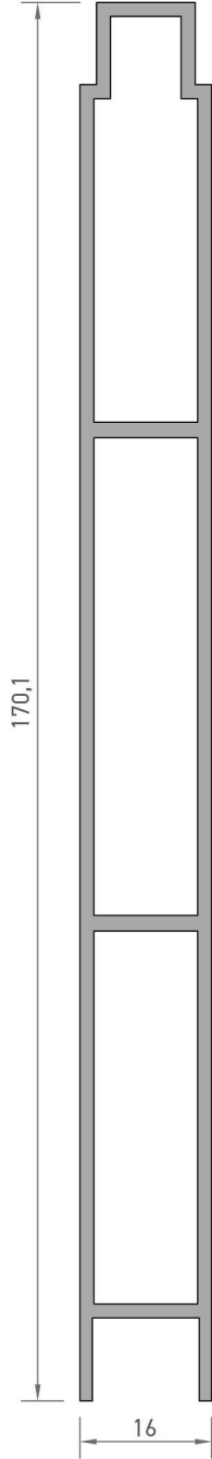
9232 TAHTA LAMBİRİ PROFİLİ 1,805 kg/mt
